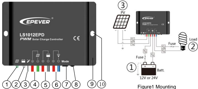
Figure1 Mounting
